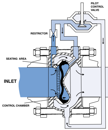
Model 100-42 Valve in Partially Open Position
